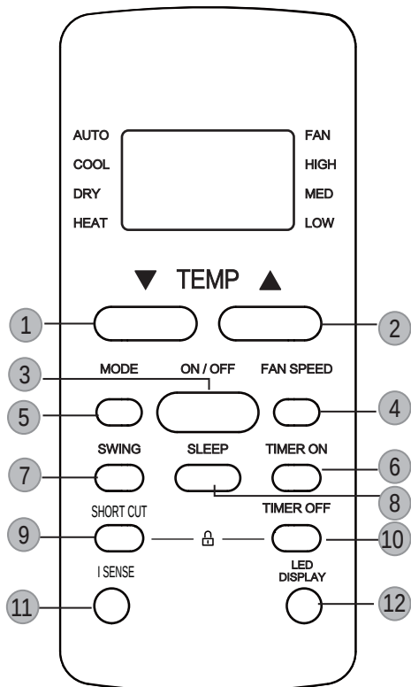
Model: RG51F/EF
